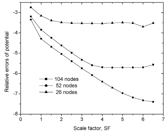
Figure 8 : Relative errors and convergence rates for the potential flow problem
