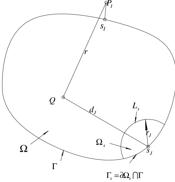
Figure 1 : The local domain centered at a node s_j and the source point of fundamental solution corresponding to a node s_l .
