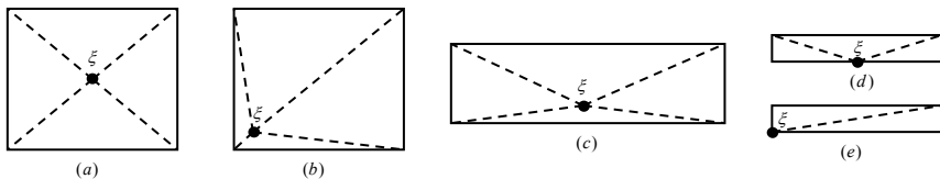
Figure 5: The conventional subdivisions of quadrilateral element.
